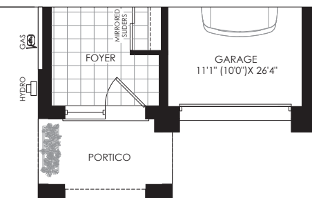
PARTIAL GROUND FLOOR PLAN ELEV. 'E'
