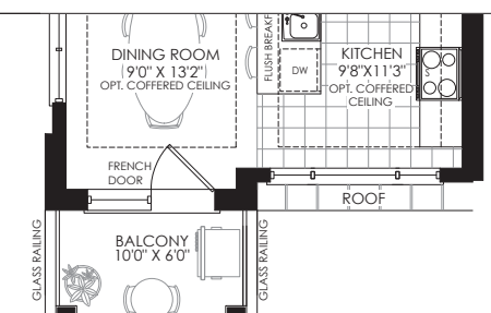
PARTIAL SECOND FLOOR PLAN ELEV. 'I'
