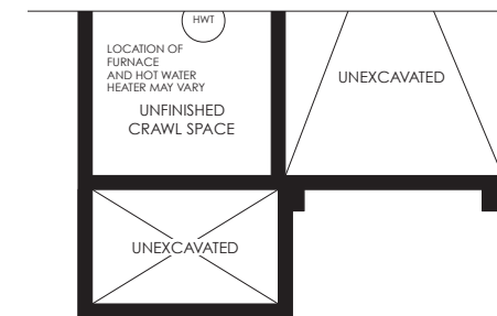
PARTIAL CRAWL SPACE PLAN ELEV. 'E'
