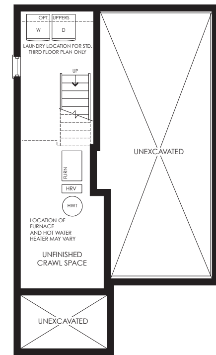
CRAWL SPACE PLAN ELEV. 'D'
