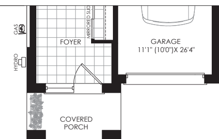
PARTIAL GROUND FLOOR PLAN ELEV. 'H'
