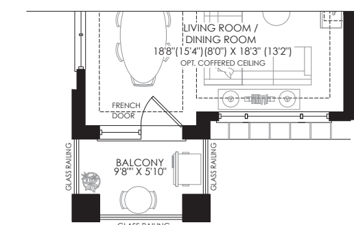
PARTIAL FLEX SECOND FLOOR PLAN ELEV. 'H'
