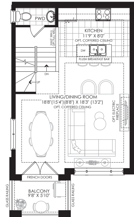
FLEX SECOND FLOOR PLAN ELEV. 'D'
